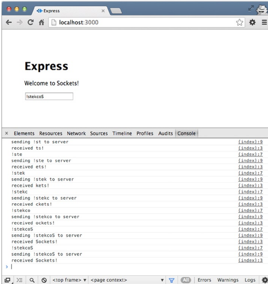
Figure 9-3. The input of IstekcoS yields Sockets!
