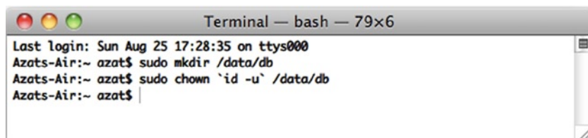
Figure 5-1. Initial setup for MongoDB: create the data directory
